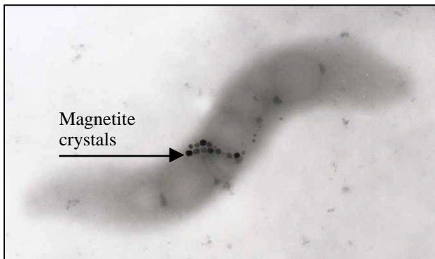
Figure 1: Transmission electron micrograph of the magnetotactic bacterium M. magnetotacticum . Opaque (electron-dense) particles are crystals of biogenic magnetite.
