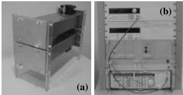
Figure 3: The REFLEX system: (a) two 1.8 GHz waveguides which fit into an incubator, and (b) the control electronics.
